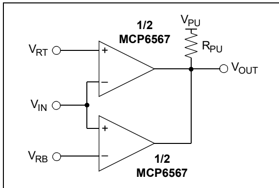
FIGURE 4-13: Windowed Comparator.
