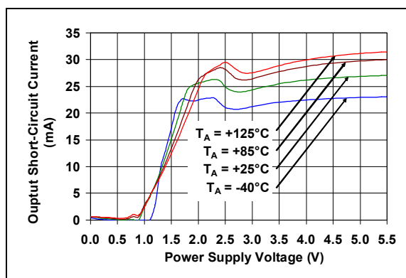
FIGURE 2-12: Output Short-Circuit Current vs. Supply Voltage.
