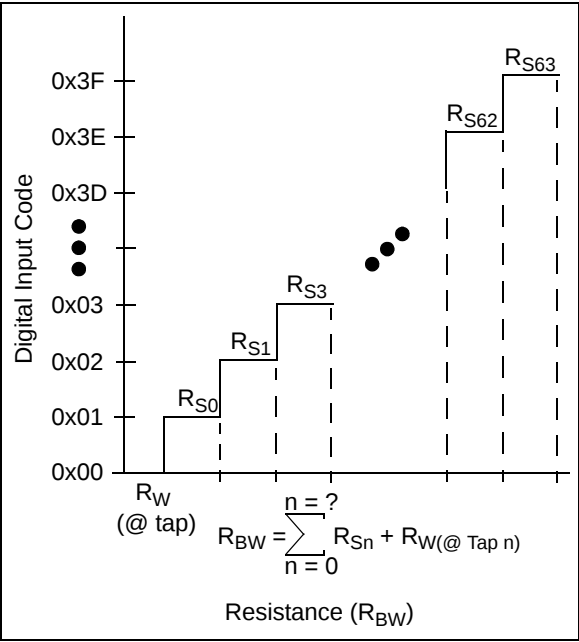
FIGURE 6-7: R_{BW}
