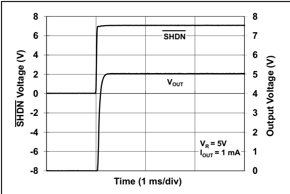
FIGURE 2-41: SHDN Response.
