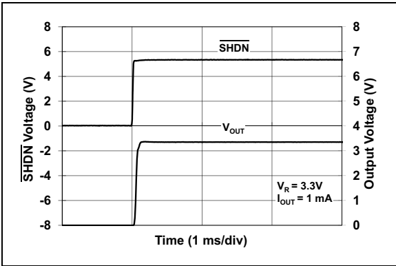
FIGURE 2-40: SHDN Response.
