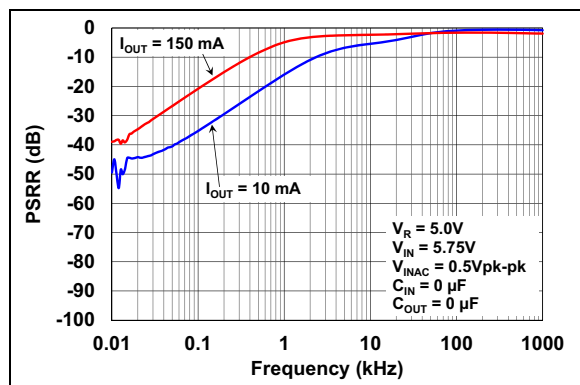
FIGURE 2-73: Power Supply Ripple Rejection vs. Frequency.
