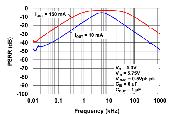
FIGURE 2-74: Power Supply Ripple Rejection vs. Frequency.
