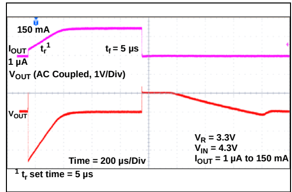
FIGURE 2-58: Dynamic Load Response.
