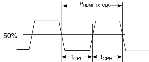
Figure 54. TMDS Clock Signal Definitions
