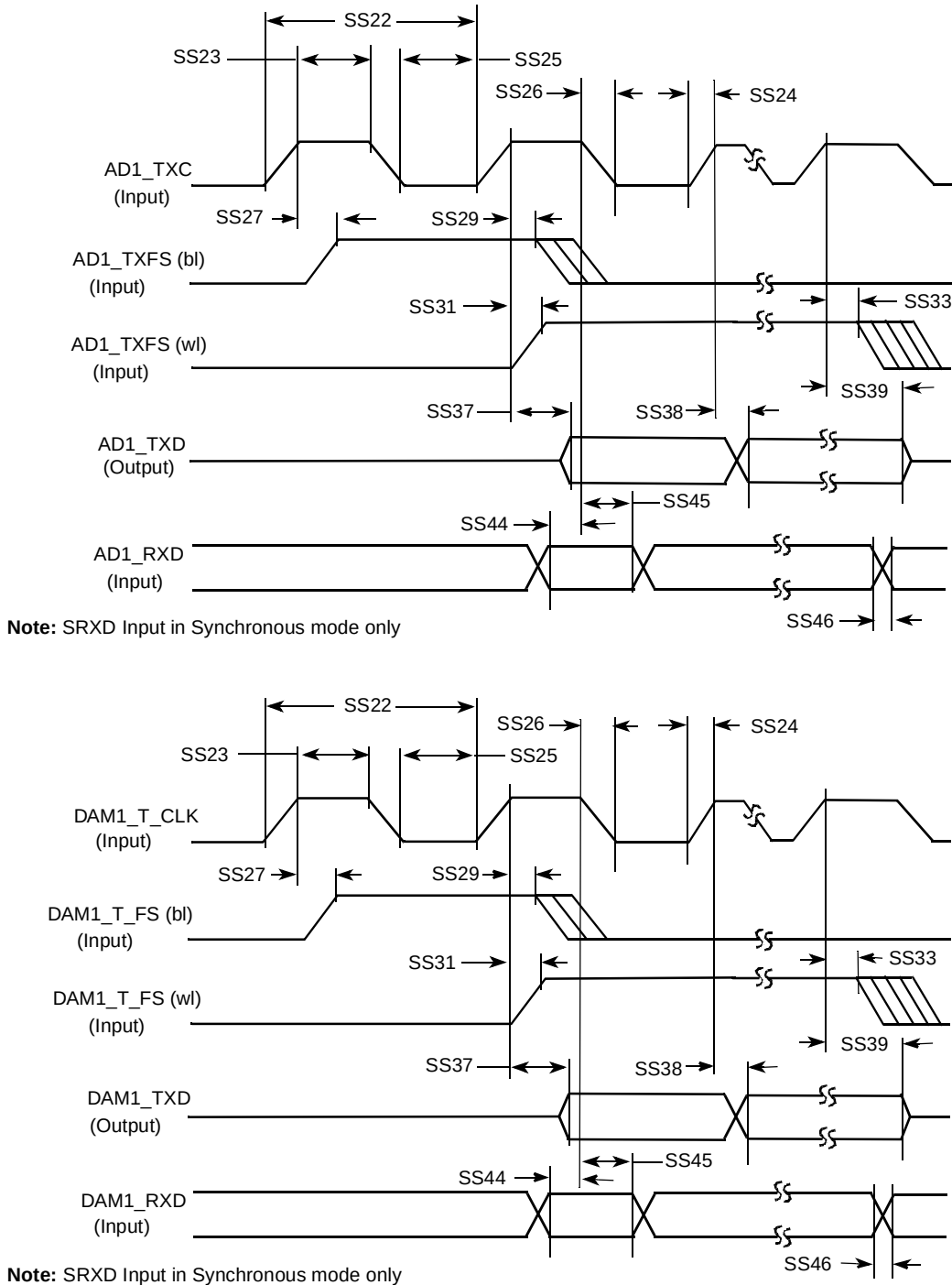
Figure 82. SSI Transmitter with External Clock Timing Diagram
