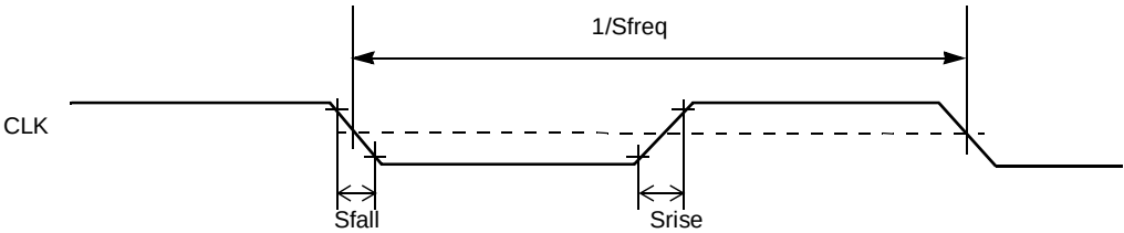
Figure 72. SIM Clock Timing Diagram
