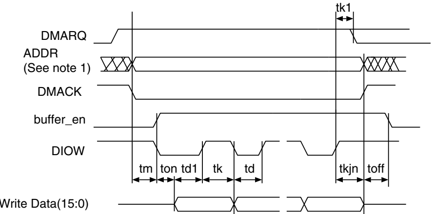
Figure 14. MDMA Write Mode Timing
