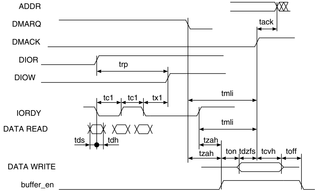
Figure 16. Timing for Host-Terminated UDMA In-Transfer
