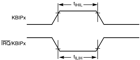
Figure 16. \overline{\text{IRQ}}/\text{KBIPx} Timing
