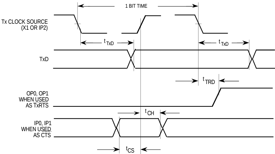
Figure 8-15. Transmit Timing
