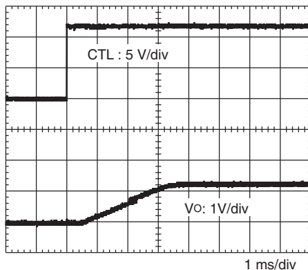
CTL Start-up Waveform
