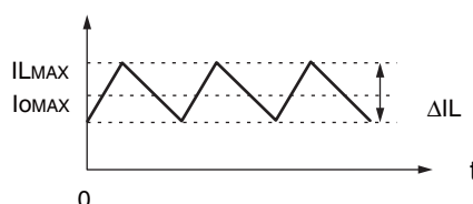
Inductor current
