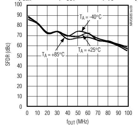
SFDR vs. f_{OUT} AND TEMPERATURE ( f_{CLK} = 200MHz , A_{OUT} = -6dB FS , I_{FS} = 20mA )
