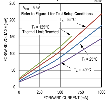
FORWARD VOLTAGE vs. FORWARD CURRENT (SOT)
