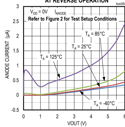
ANODE CURRENT AT REVERSE OPERATION
