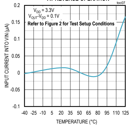
ANODE CURRENT AT REVERSE OPERATION
