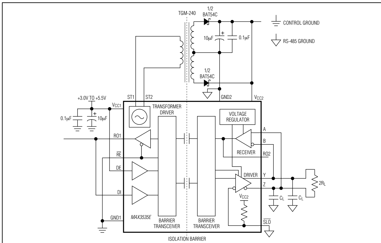
Figure 5. Self-Oscillating Configuration
