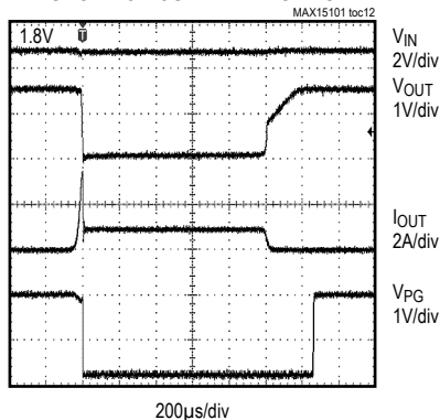
SHORT-CIRCUIT WAVEFORMS
