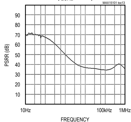
PSRR vs. FREQUENCY (I LOAD = 0.5A)
