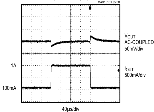
1A LOAD-TRANSIENT RESPONSE (C OUT = 10μF)
