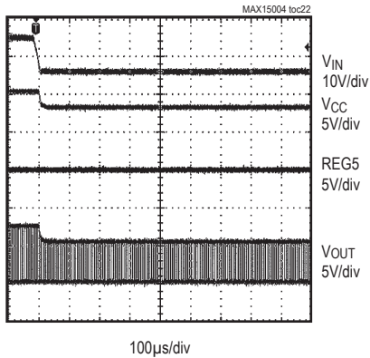
HICCUP MODE FOR FLYBACK CIRCUIT (FIGURE 7)
