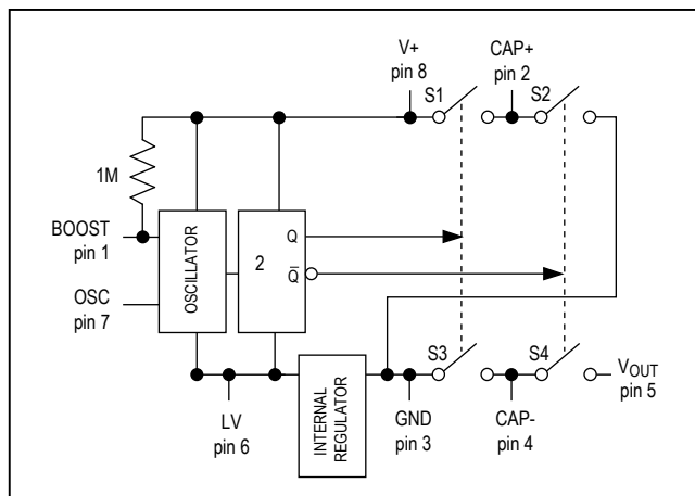
Figure 4. MAX1044 and ICL7660 Functional Diagram
