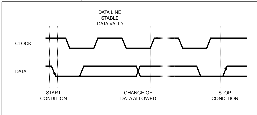
Figure 7: Acknowledgement sequence
