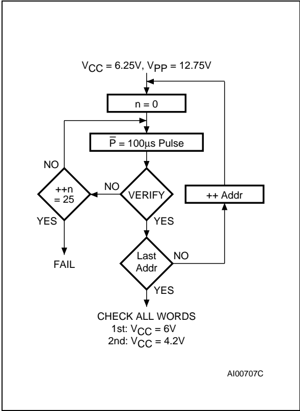
Figure 9. Programming Flowchart
