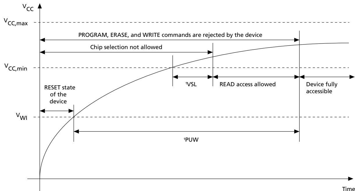
Figure 20: Power-Up Timing
