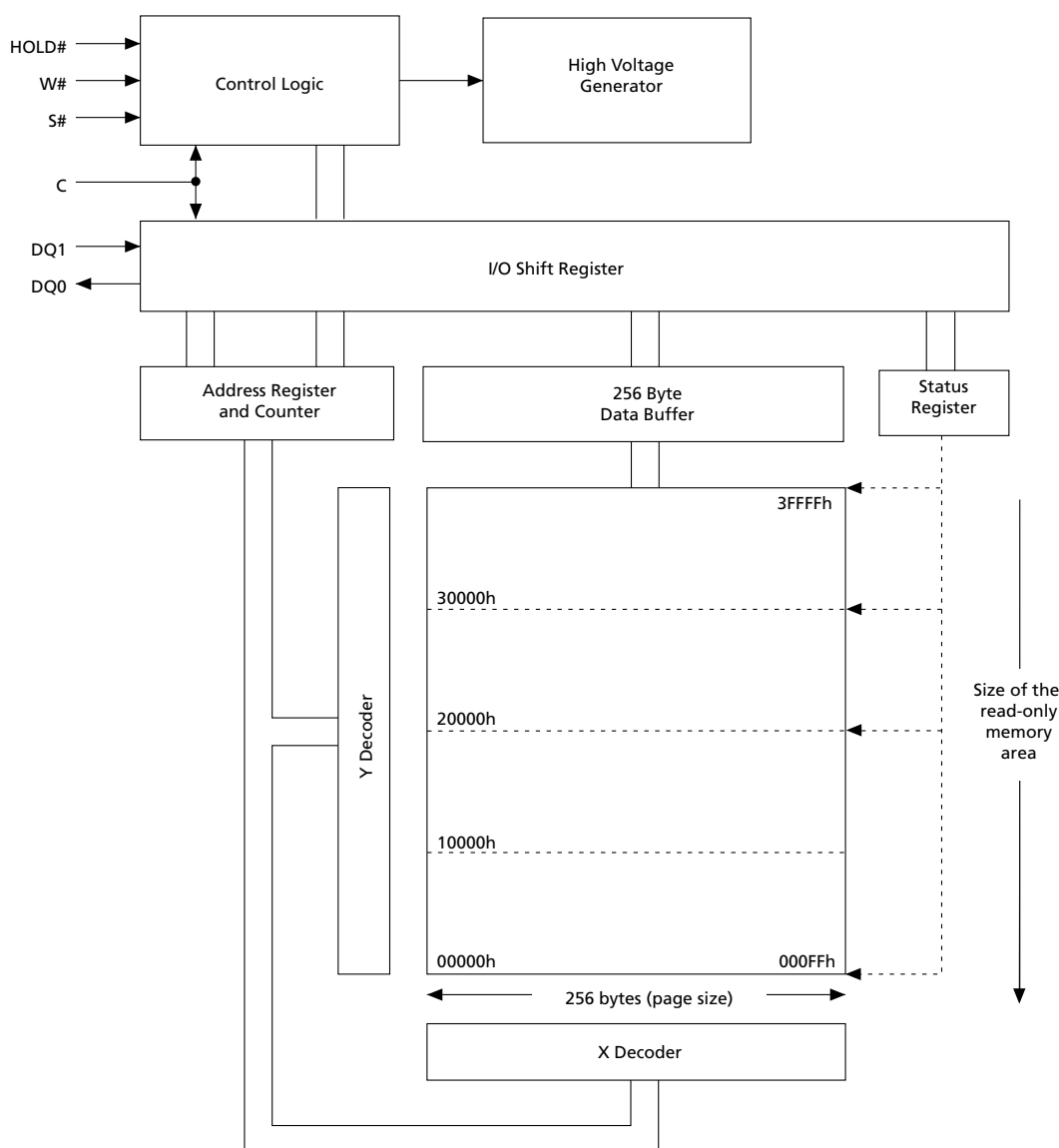
Figure 6: Block Diagram
