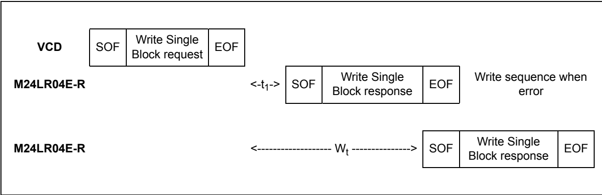
Figure 55. Write Single Block frame exchange between VCD and M24LR04E-R
