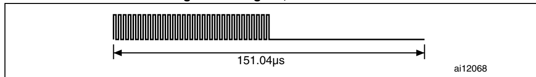
Figure 27. Logic 0, low data rate
