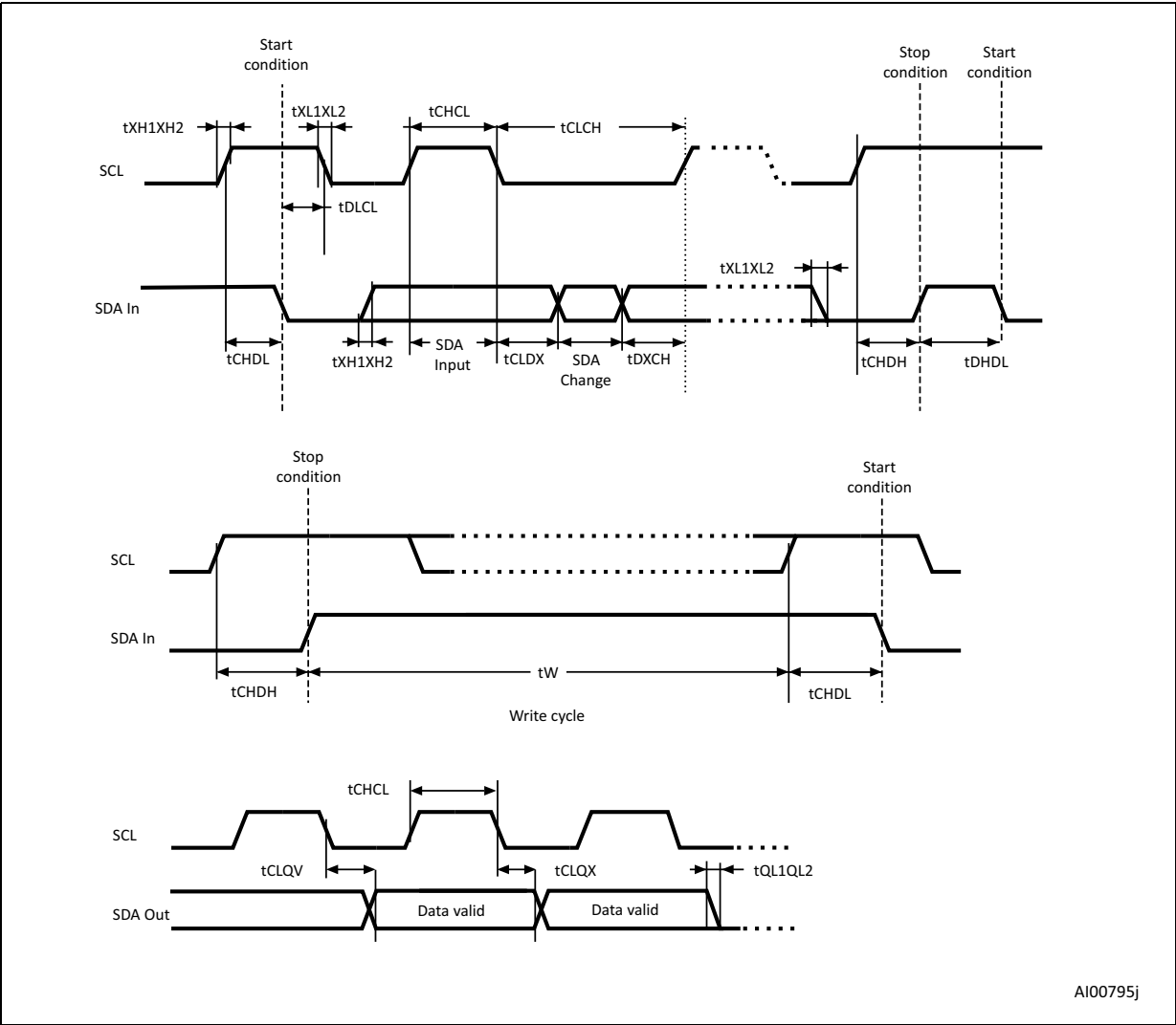
Figure 14. AC waveforms
