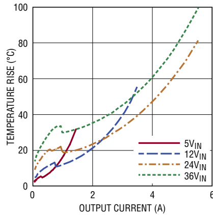
Temperature Rise vs Output Current ( 12V_{OUT} )
