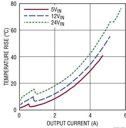
Temperature Rise vs Output Current ( 3.3V_{OUT} )
