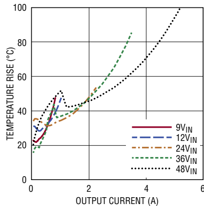
Temperature Rise vs Output Current ( 36V_{OUT} )
