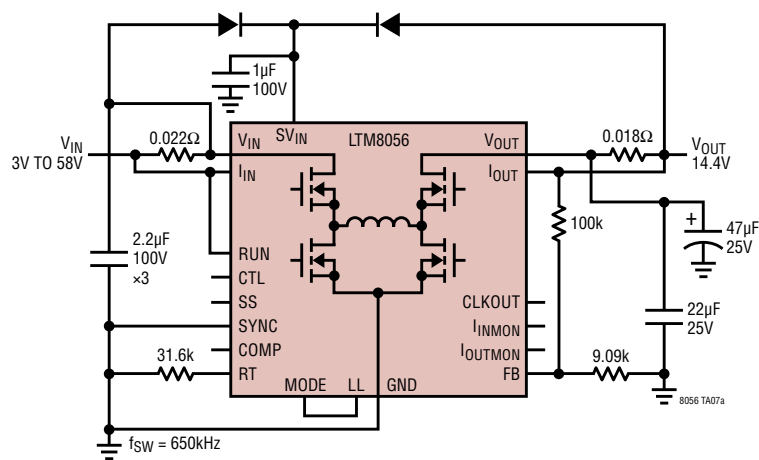
14.4V, 3A Lead-Acid Battery Charger Input Current Limited to 2A
