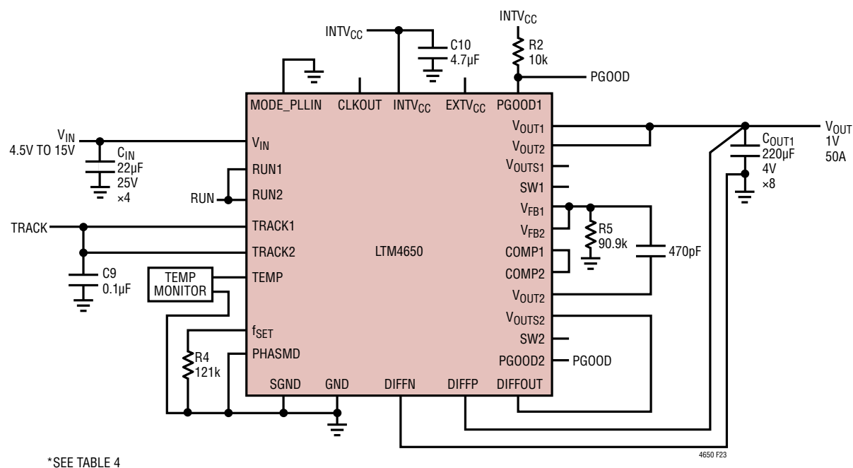
Figure 23. LTM4650 2-Phase, 1V at 50A Design
