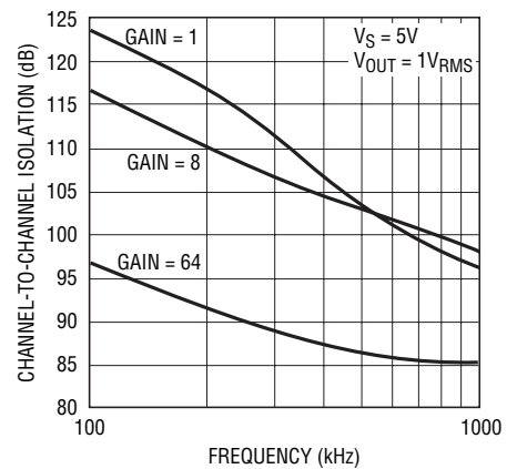
LTC6912-2 Channel Isolation vs Frequency
