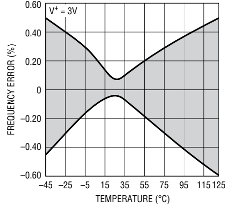
Typical Frequency Error vs Temperature, DFN Package (Note 3)
