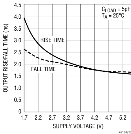
Typical Output Rise/Fall Time vs Supply
