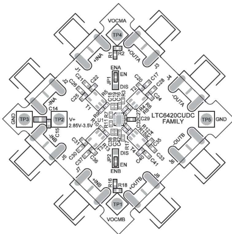
NOTES: UNLESS OTHERWISE SPECIFIED [1] DO NOT STUFF [2] VERSION U1 R5, R9, R10, R13 T1, T3 -C LTC6420CUDC-20 NONE TCM4-19+ -G LTC6421CUDC-20 NONE TCM4-19+ 642020 F04b
