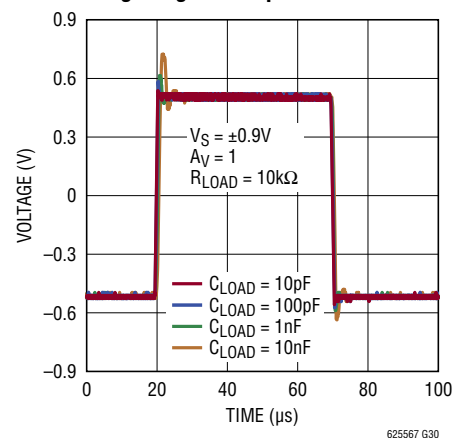
Large-Signal Response
