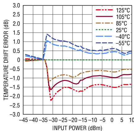
Linearity Error Temperature Variation from 25°C at 38GHz
