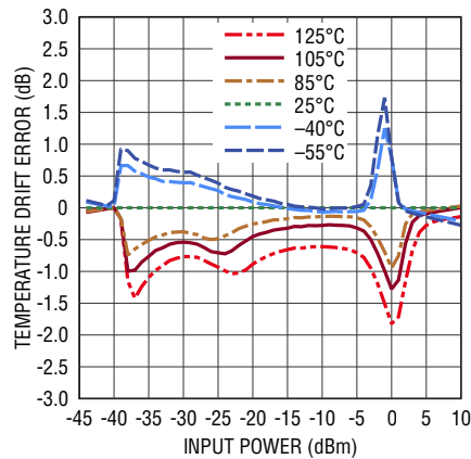
Linearity Error Temperature Variation from 25°C at 28GHz
