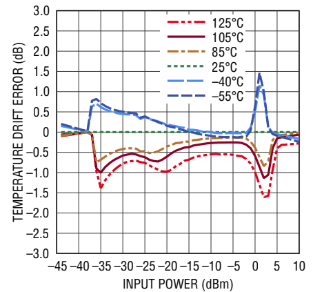
Linearity Error Temperature Variation from 25°C at 26GHz
