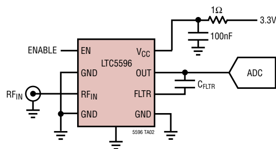
100MHz to 40GHz Power Measurement
