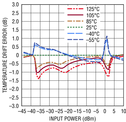
Linearity Error Temperature Variation from 25^\circ C at 2.14GHz
