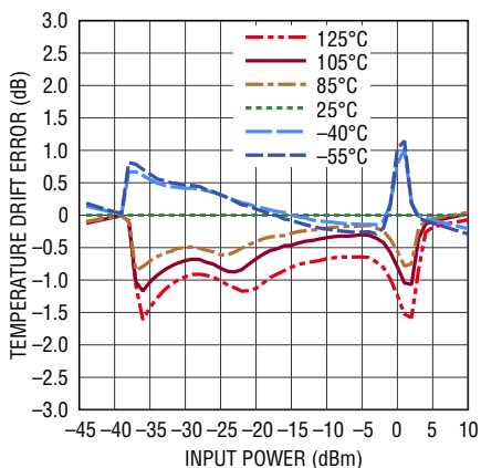
Linearity Error Temperature Variation from 25^\circ C at 10GHz
