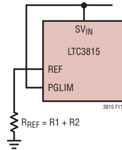
Figure 11a. PGOOD Window Set to \pm 10\% Default
