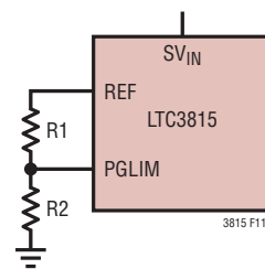
Figure 11b. PGOOD Window Set By R1/R2
