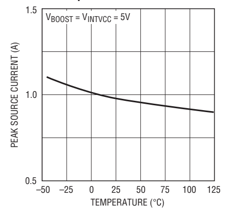
Driver Peak Source Current vs Temperature
