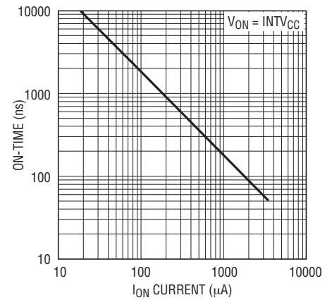
On-Time vs I_{ON} Current
