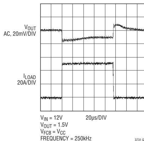
Transient Load Current Response: 0 Amp to 50 Amp (Circuit of Figure 14)
