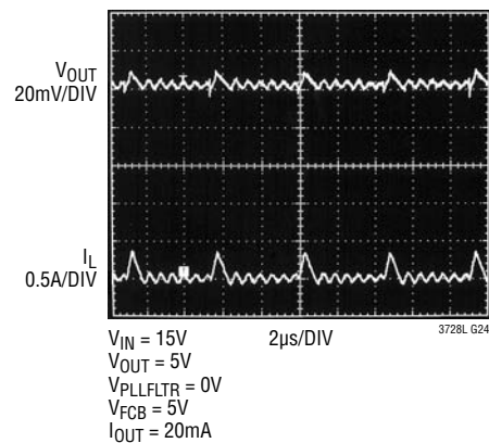
Constant-Frequency (Burst Inhibit) Operation (Figure 13)
