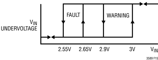
Figure 15. UV Detection Hard Reset and Warning Levels
