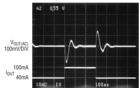
V_{OUT} Transient Response
