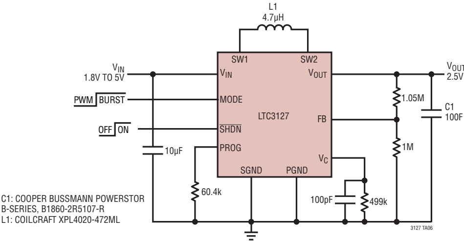
Single Supercapacitor Charger (1000mA Max Input Current)
