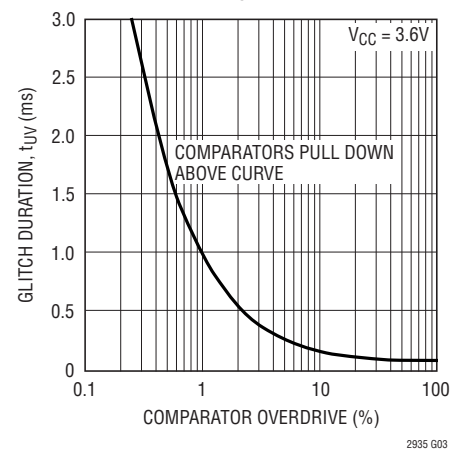
Comparator Undervoltage Glitch Immunity
