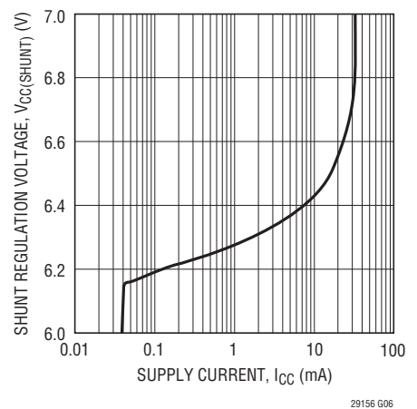
Shunt Regulation Voltage vs Supply Current
