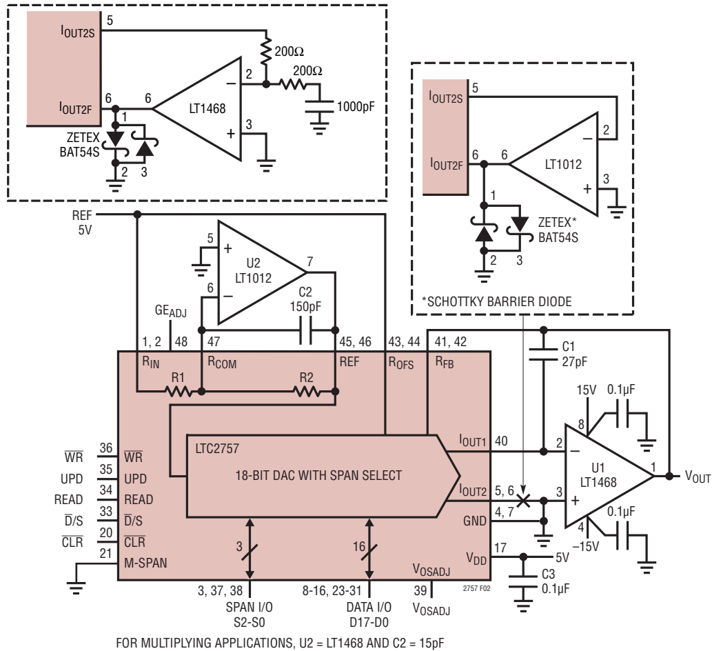
Figure 2. Basic Connections for SoftSpan V_{OUT} DAC with Two Optional Circuits for Driving I_{OUT2} from GND with a Force/Sense Amplifier
