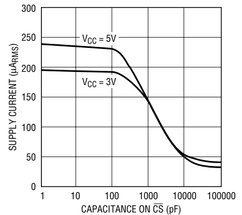
Figure 15. \overline{CS} Capacitance vs Supply Current
