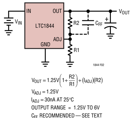
Figure 2. Adjustable Operation
