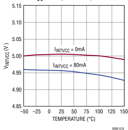
INTV CC Voltage vs Temperature
