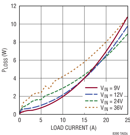
Power Loss vs Load Current
