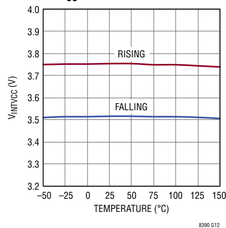
INTV CC UVLO Threshold
