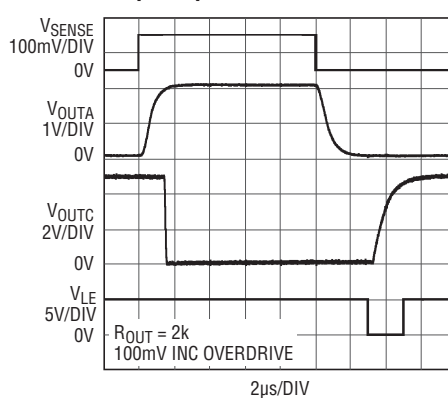
Step Response
