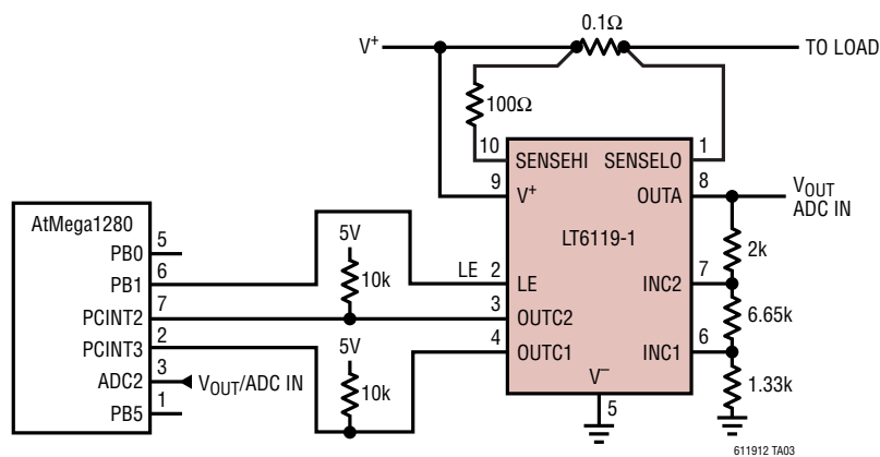
MCU Interfacing with Hardware Interrupts
