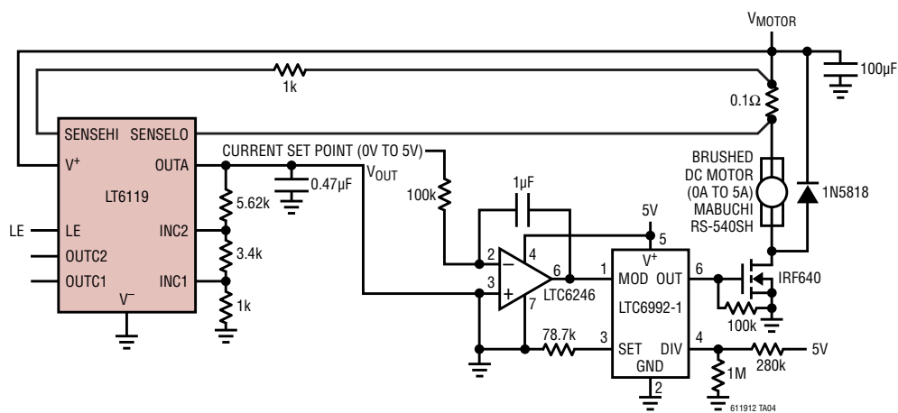
Simplified DC Motor Torque Control
