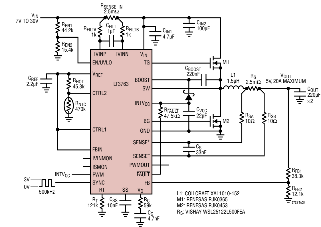
20A, Synchronized, 5V Regulator
