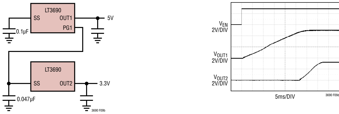
(9b) Output Sequencing
