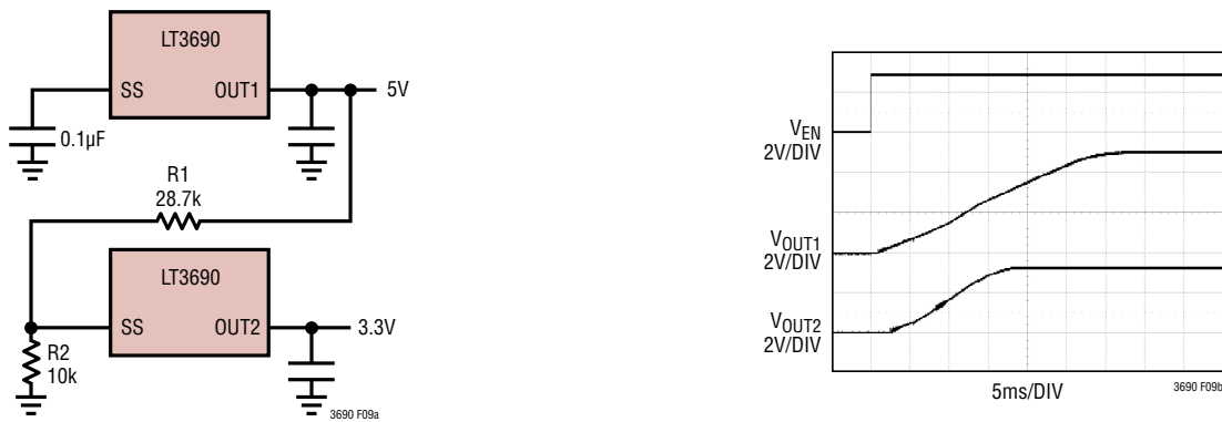
(9a) Coincident Start-Up
