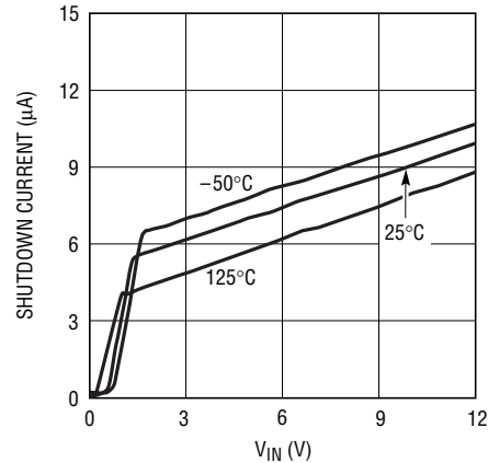
Shutdown Current ( V_{CTRL} = 0\text{V} )
