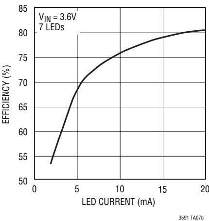
Conversion Efficiency
