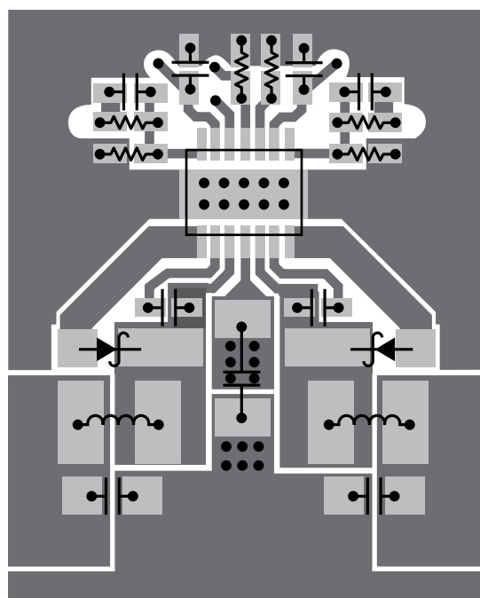
Figure 13. Sample PCB Layout (Top Layer Only)
