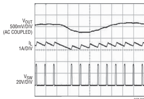
Figure 4. Operation above V_{IN(MAX)} . Output Ripple and Peak Inductor Current Increases
