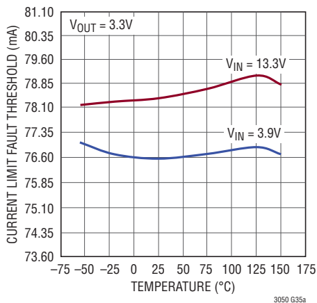
External Current Limit R_{I\text{MAX}} = 1.5\text{k}
